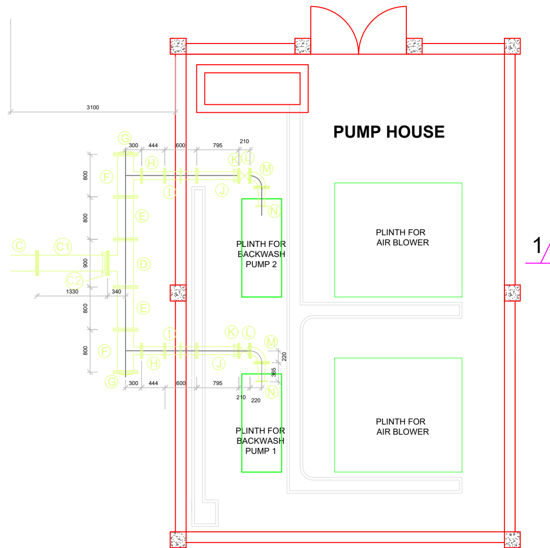
BACKWASH PUMPS SUCTION PIPEWORK DETAILS PLAN
