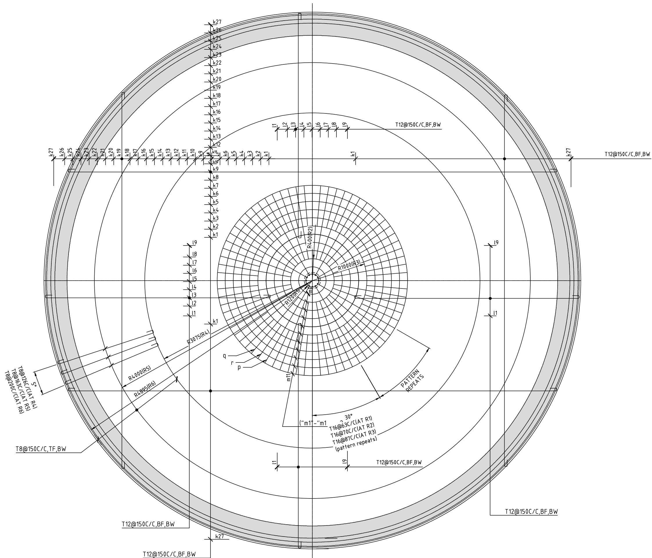
ROOF REINFORCEMENT SCALE 1:25
